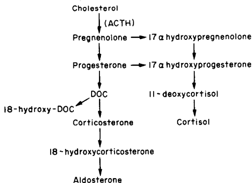
Fig. 1. Biosynthesis of corticosteroids.
